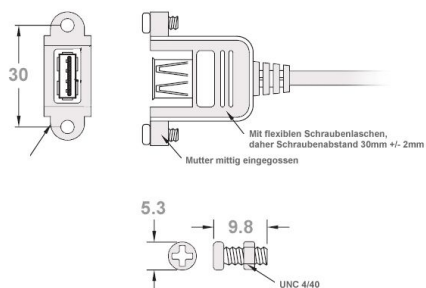
USB 2.0 A Buchse / female / femelle
